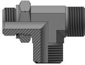
90° ADAPTOR FEMALE ORFS - ADJUSTABLE MALE BSPP WITH O-RING PAG. 285
