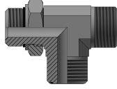
90° ADAPTOR FEMALE ORFS - ADJUSTABLE METRIC MALE WITH O- RING PAG. 286
