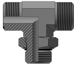
ADJUSTABLE BRANCH TEE MALE ORFS - MALE UNF WITH O-RING PAG. 283
