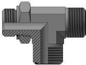
ADJUSTABLE BRANCH TEE MALE ORFS - MALE UNF WITH O-RING PAG. 283
